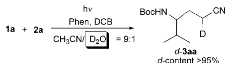
Scheme 4. Deuterium Incorporation Experiment Using D 2 O
