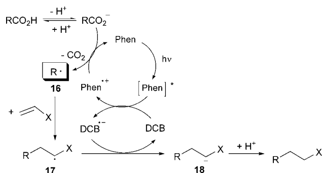
Scheme 5. Plausible Mechanism
